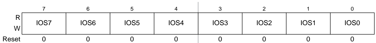
Figure 7-3. Timer Input Capture/Output Compare Register (TIOS)
